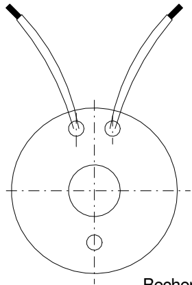
Becher 321810 (Ring-Wandler)
