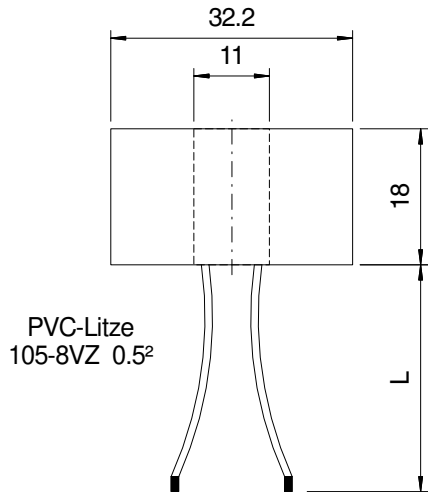
Becher 321810 (Ring-Wandler)
