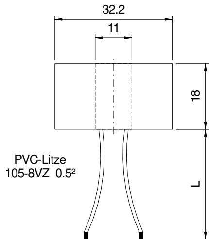
Becher 321810 (Ring-Wandler)
