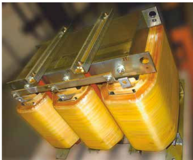
High efficiency 100kVA transformer for photovoltaic plant.
