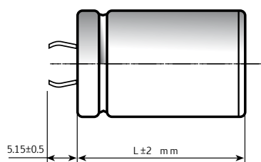
3 PIN CAPACITOR
