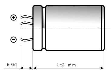
4 PIN CAPACITOR
